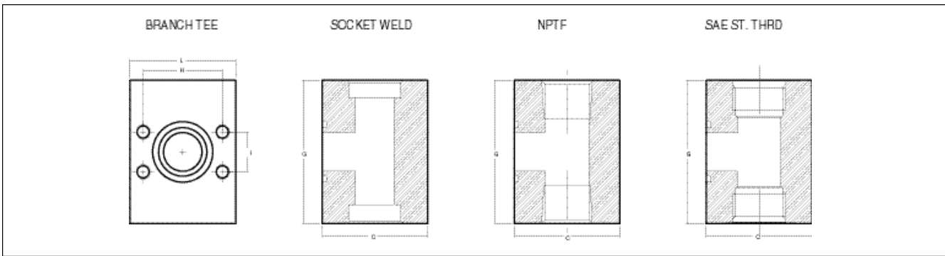
Branch Tees
