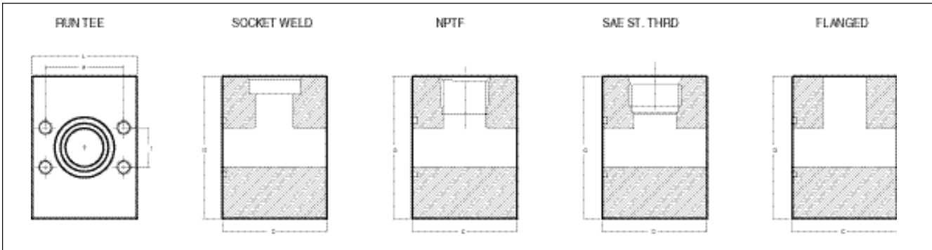
Run Tees
