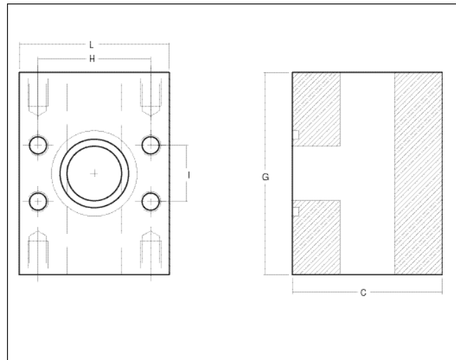
Flanged Branch Tee
